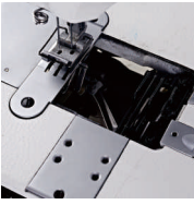
弯针机构 Curved needle construction
