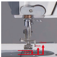
压脚高度可随意设定 Stepping motor lifts the presser foot
