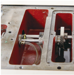
密封式齿轮箱 closed type gear box
