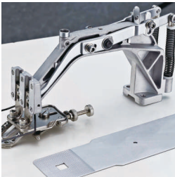
套结钉扣简易快速更换装置 Simple and quick replacement device for fastening pin buckle
