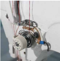
断线检测装置 Disconnection detection device
