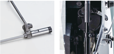
特殊处理超耐磨下轴系统 Special treatment, super wear, lower shaft system 无污染干式润滑，镀黑金钢针杆（头部特写） No pollution dry lubrication, black plating Steel needle rod (head feature)
