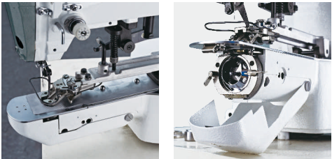
大范围可调节扣夹 big range adjustable retaining clip 高精度进口耐磨摆梭 High precision imported wear-resistant shuttle
