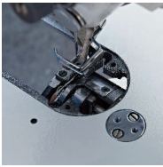
圆刀剪线 Round thread-trimmer
